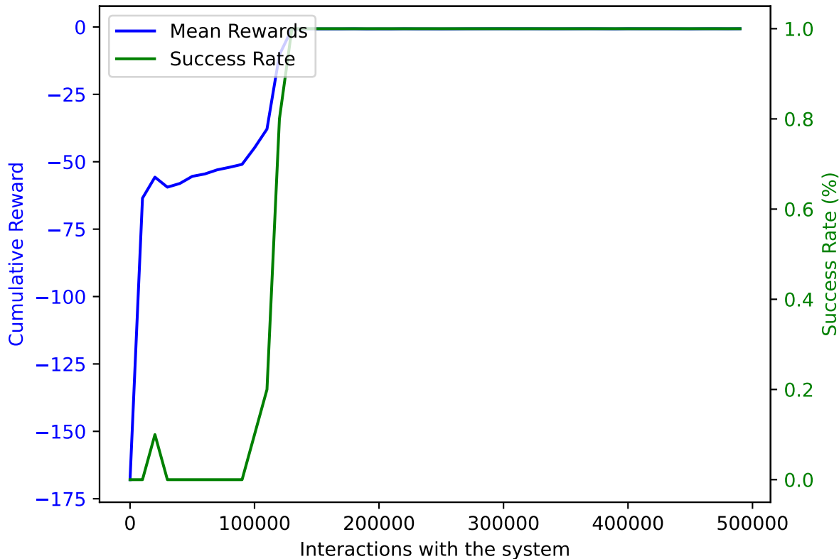
PPO on AWAKE with DoF: 5 and trained on 490000 samples averaged over 10 validation episodes
