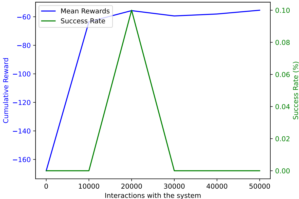
PPO on AWAKE with DoF: 5 and trained on 50000 samples averaged over 10 validation episodes
