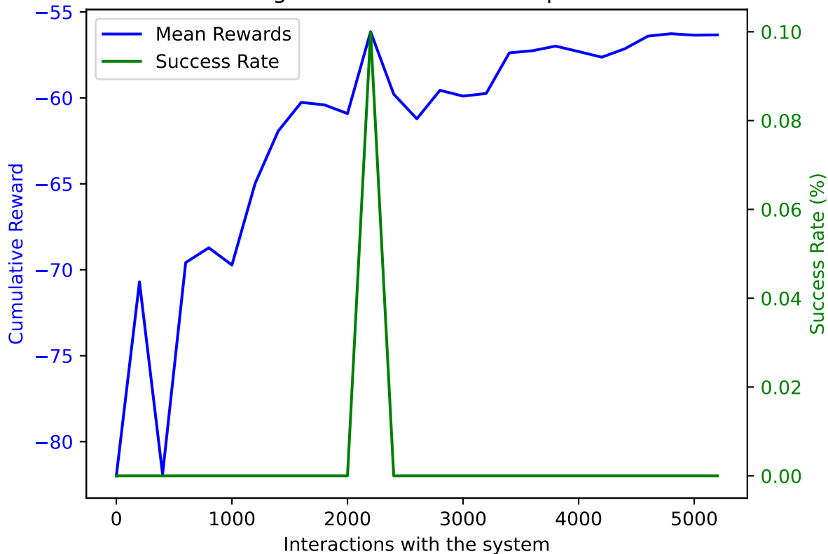
PPO on AWAKE with DoF: 5 and trained on 5200 samples averaged over 10 validation episodes
