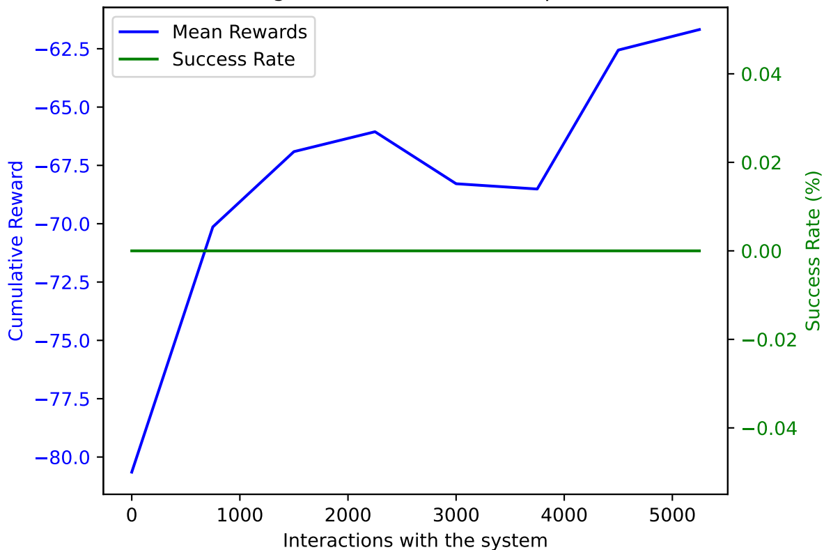
PPO on AWAKE with DoF: 5 and trained on 5250 samples averaged over 10 validation episodes
