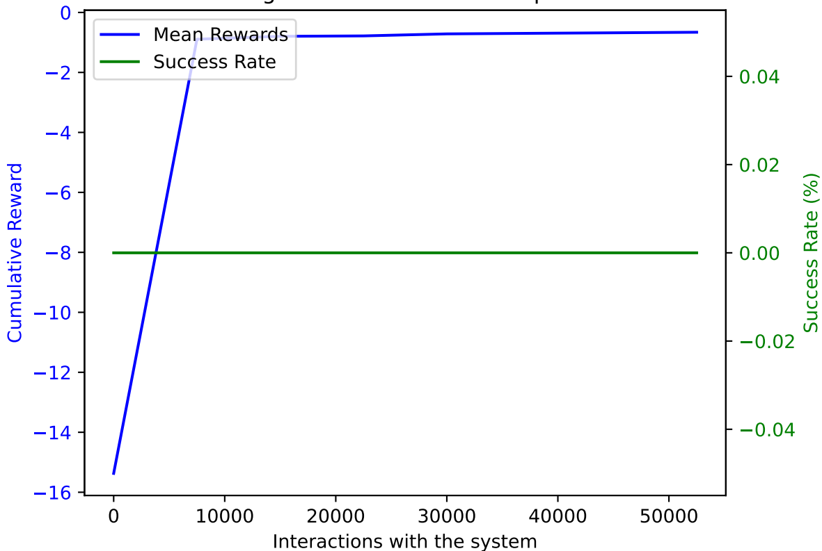
PPO on AWAKE with DoF: 5 and trained on 52500 samples averaged over 10 validation episodes
