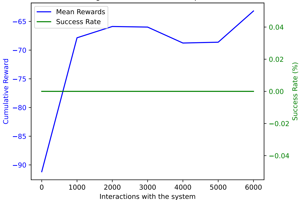
PPO on AWAKE with DoF: 5 and trained on 6000 samples averaged over 10 validation episodes
