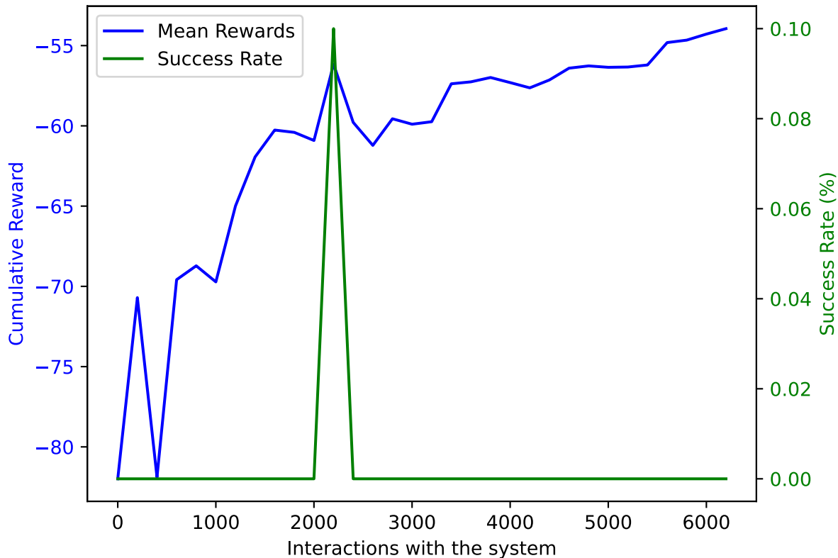
PPO on AWAKE with DoF: 5 and trained on 6200 samples averaged over 10 validation episodes
