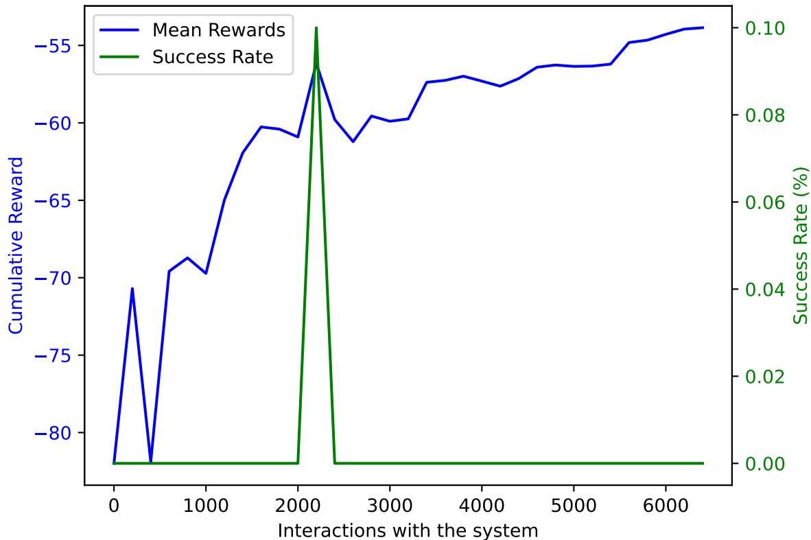
PPO on AWAKE with DoF: 5 and trained on 6400 samples averaged over 10 validation episodes
