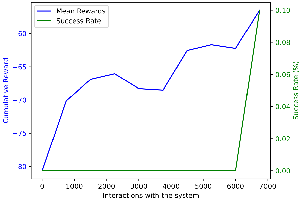
PPO on AWAKE with DoF: 5 and trained on 6750 samples averaged over 10 validation episodes
