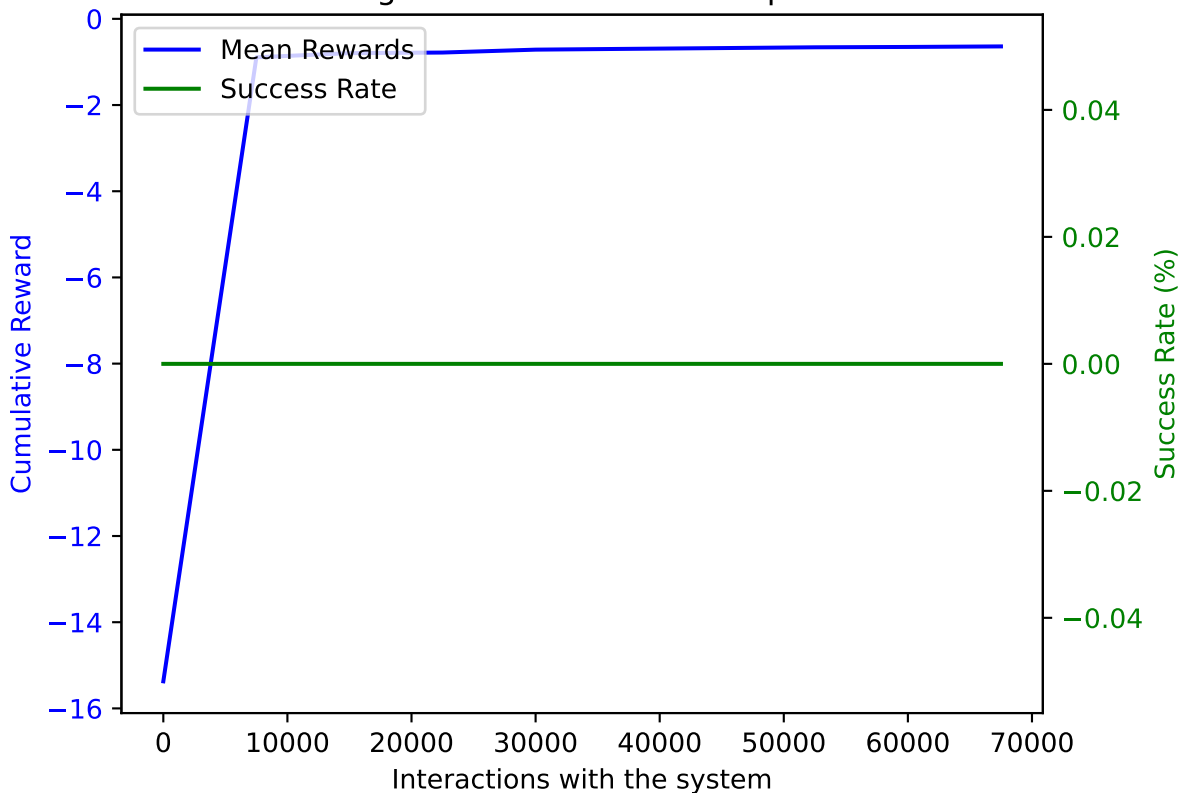
PPO on AWAKE with DoF: 5 and trained on 67500 samples averaged over 10 validation episodes
