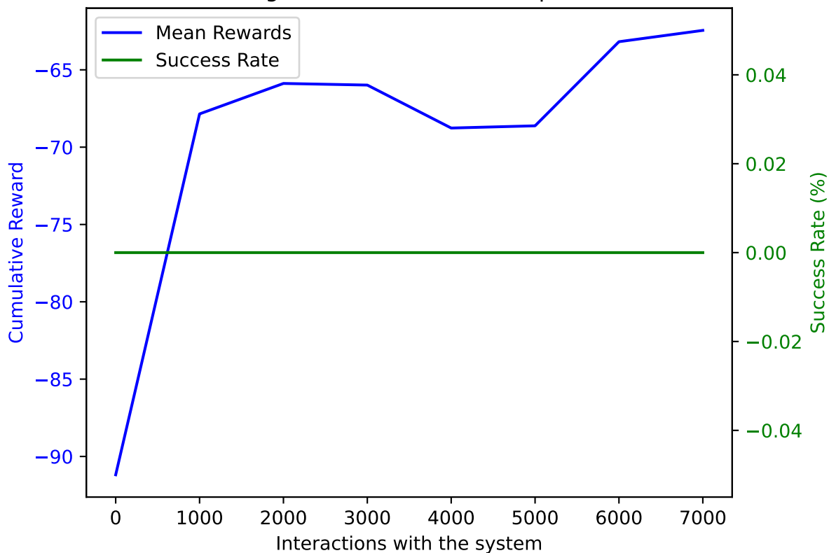
PPO on AWAKE with DoF: 5 and trained on 7000 samples averaged over 10 validation episodes
