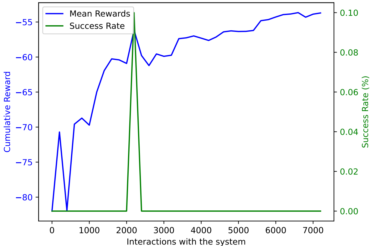
PPO on AWAKE with DoF: 5 and trained on 7200 samples averaged over 10 validation episodes
