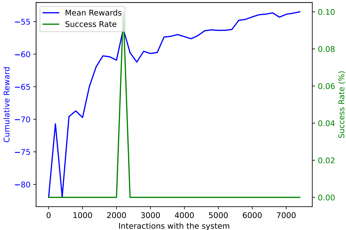
PPO on AWAKE with DoF: 5 and trained on 7400 samples averaged over 10 validation episodes
