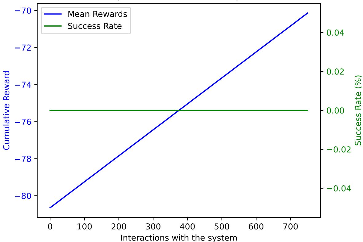
PPO on AWAKE with DoF: 5 and trained on 750 samples averaged over 10 validation episodes
