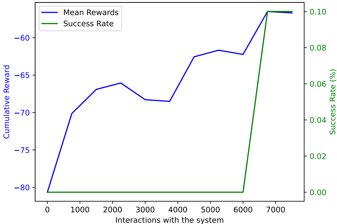
PPO on AWAKE with DoF: 5 and trained on 7500 samples averaged over 10 validation episodes
