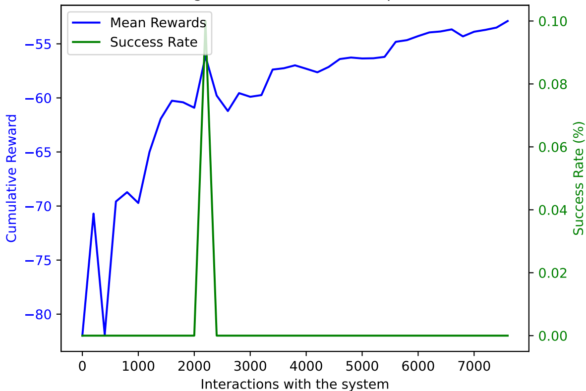
PPO on AWAKE with DoF: 5 and trained on 7600 samples averaged over 10 validation episodes
