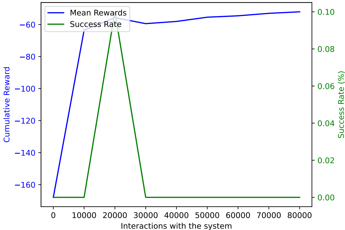
PPO on AWAKE with DoF: 5 and trained on 80000 samples averaged over 10 validation episodes
