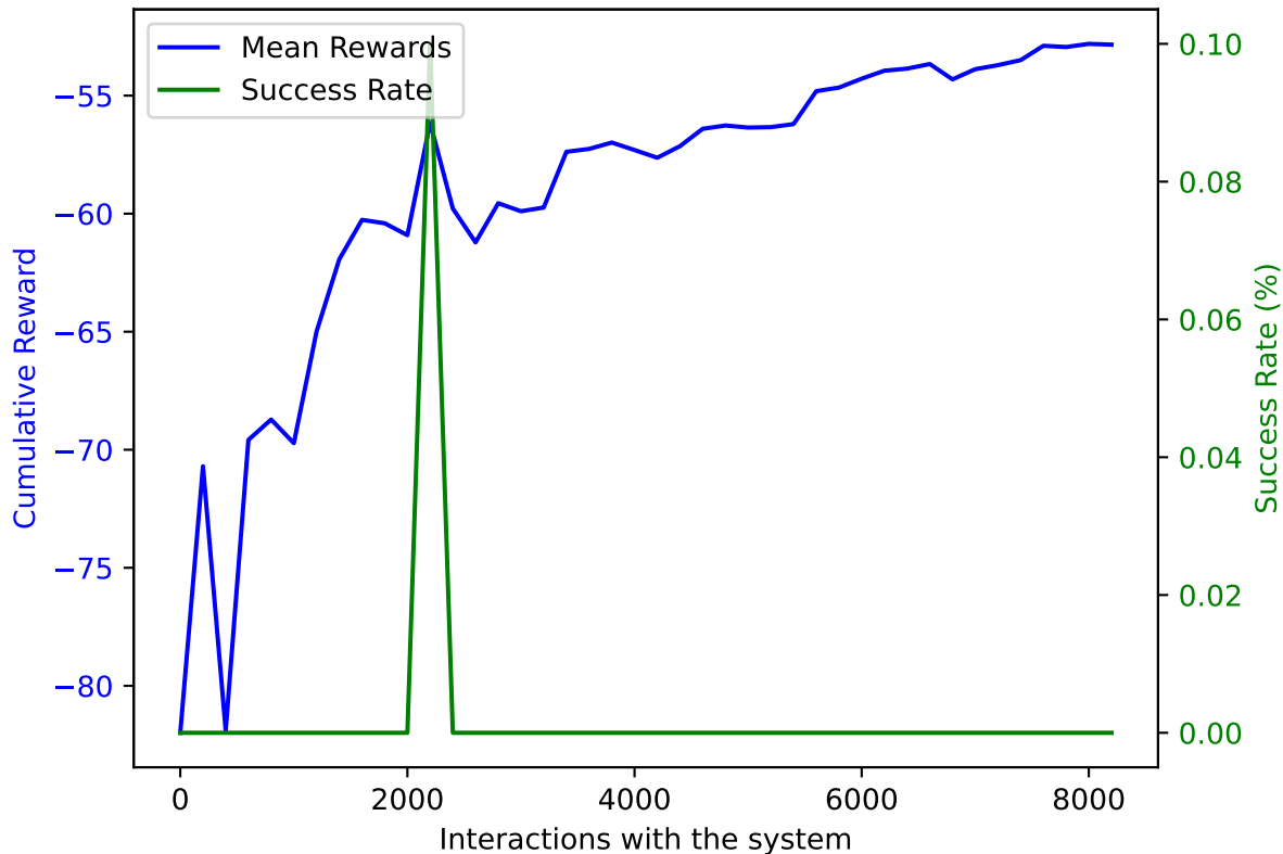
PPO on AWAKE with DoF: 5 and trained on 8200 samples averaged over 10 validation episodes
