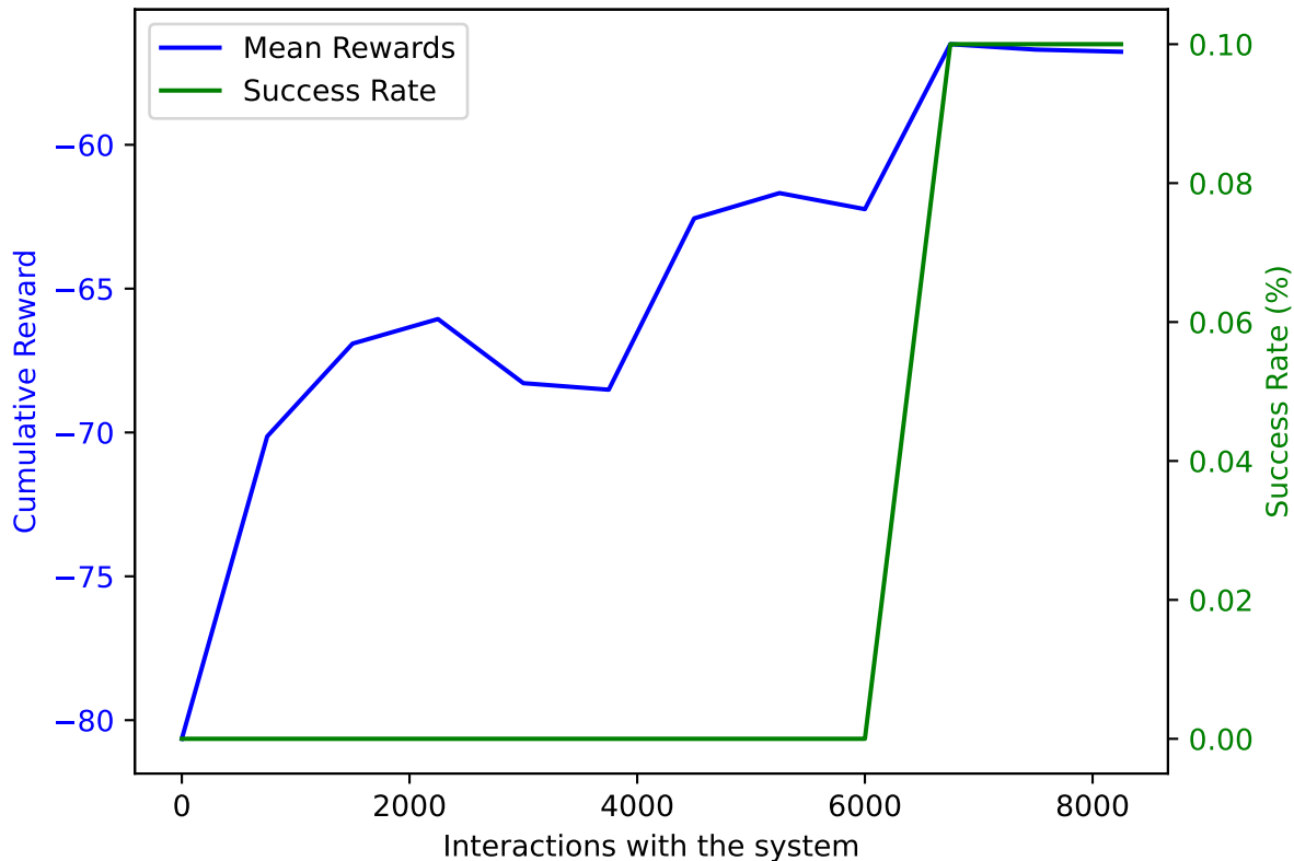
PPO on AWAKE with DoF: 5 and trained on 8250 samples averaged over 10 validation episodes
