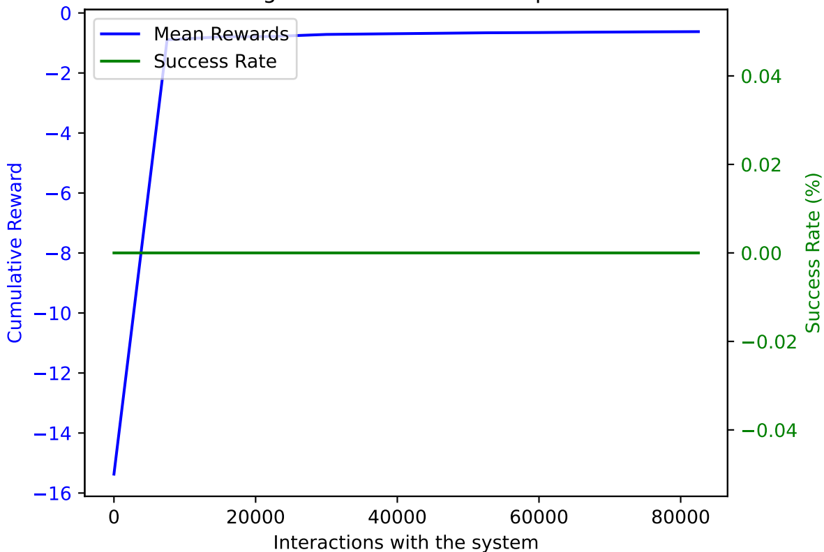
PPO on AWAKE with DoF: 5 and trained on 82500 samples averaged over 10 validation episodes
