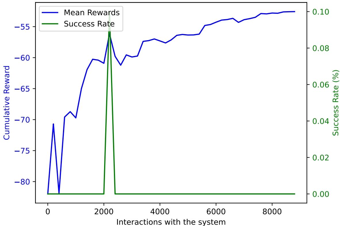
PPO on AWAKE with DoF: 5 and trained on 8800 samples averaged over 10 validation episodes
