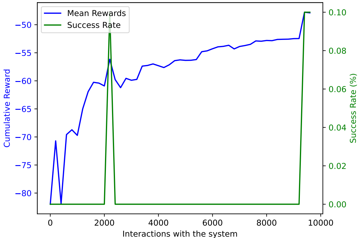
PPO on AWAKE with DoF: 5 and trained on 9600 samples averaged over 10 validation episodes
