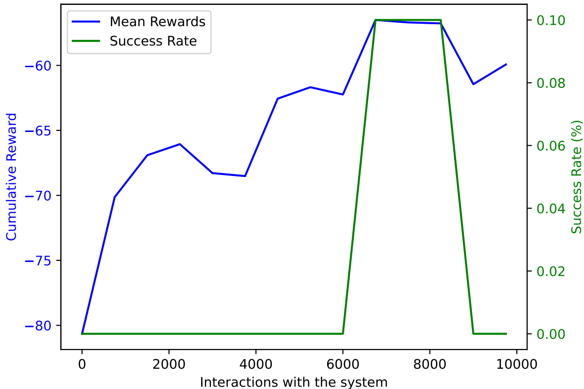
PPO on AWAKE with DoF: 5 and trained on 9750 samples averaged over 10 validation episodes
