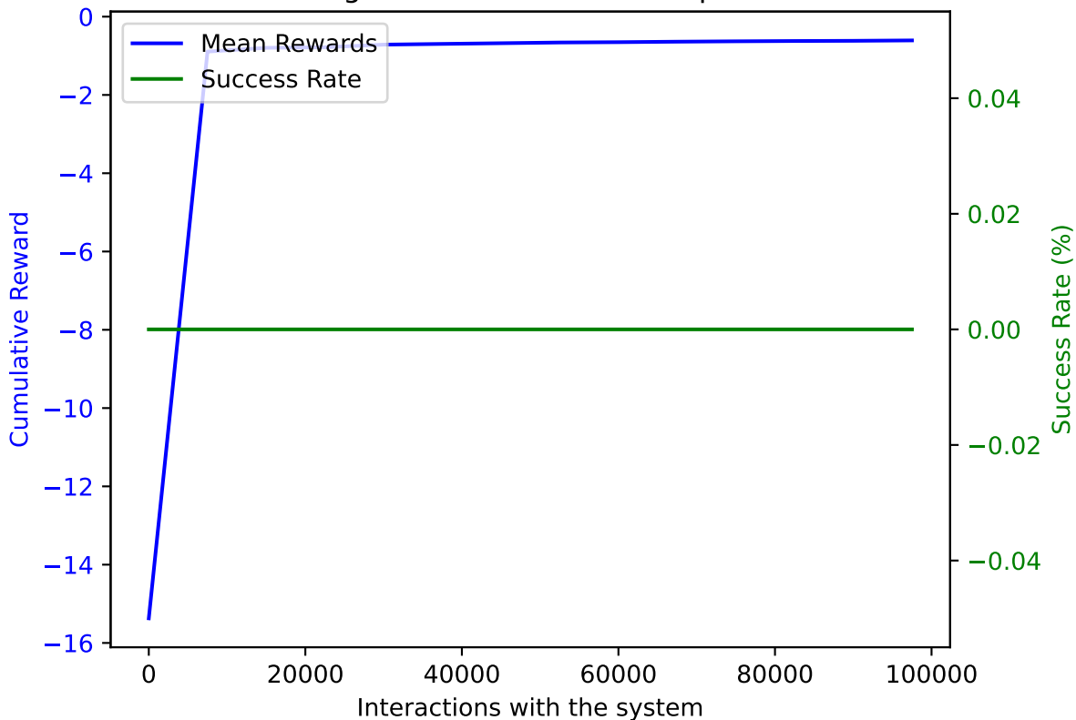
PPO on AWAKE with DoF: 5 and trained on 97500 samples averaged over 10 validation episodes
