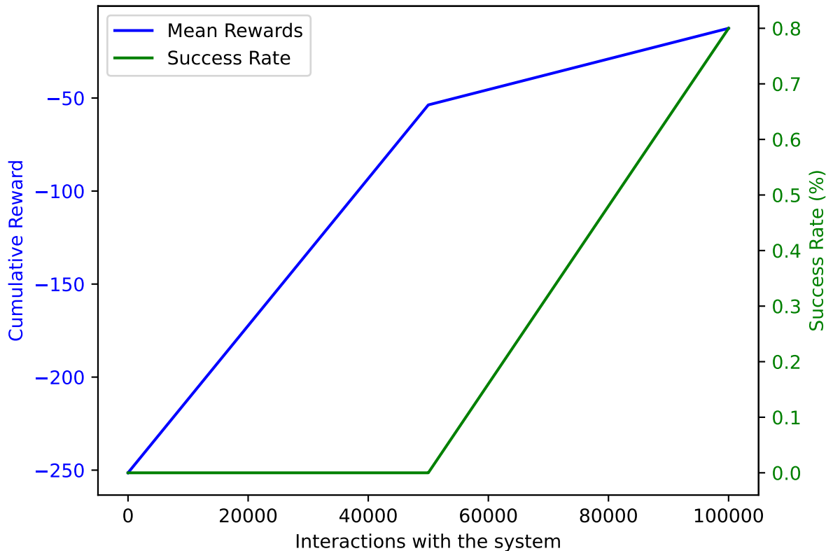
TRPO on AWAKE with DoF: 5 and trained on 100000 samples averaged over 10 validation episodes
