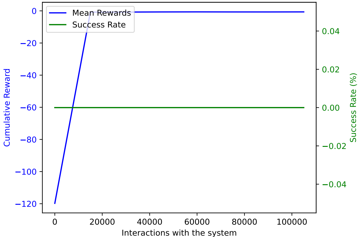
TRPO on AWAKE with DoF: 5 and trained on 105000 samples averaged over 10 validation episodes
