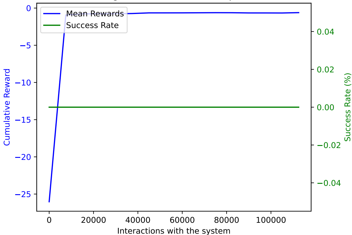
TRPO on AWAKE with DoF: 5 and trained on 112500 samples averaged over 10 validation episodes
