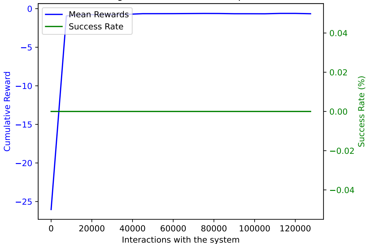
TRPO on AWAKE with DoF: 5 and trained on 127500 samples averaged over 10 validation episodes
