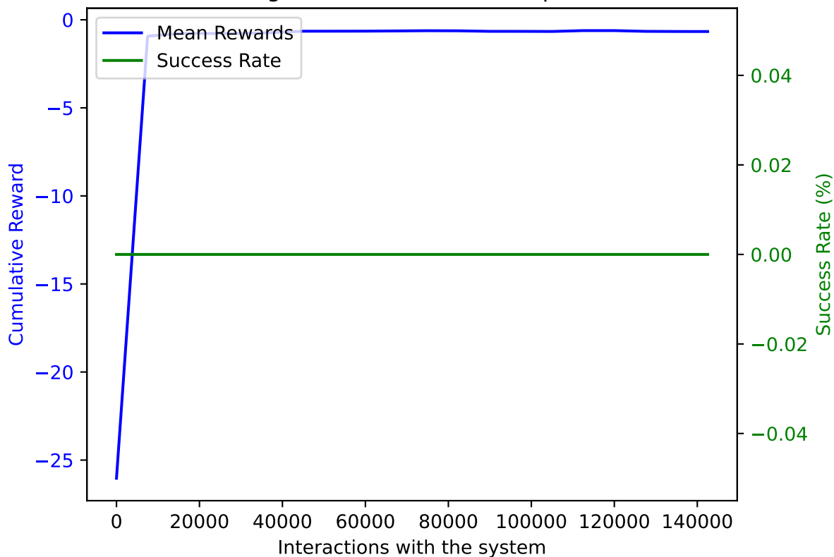
TRPO on AWAKE with DoF: 5 and trained on 142500 samples averaged over 10 validation episodes
