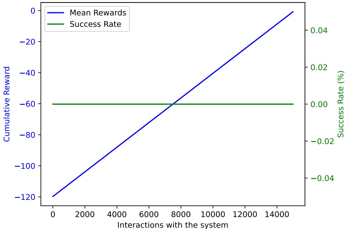
TRPO on AWAKE with DoF: 5 and trained on 15000 samples averaged over 10 validation episodes
