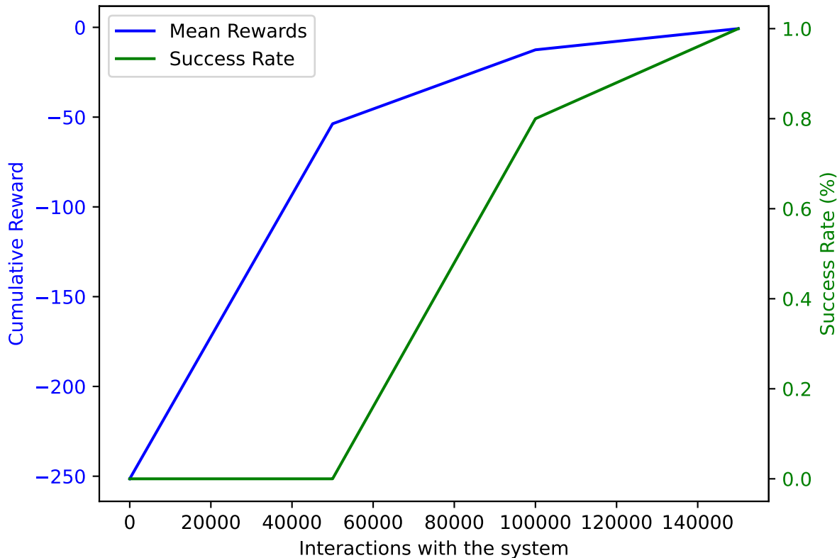
TRPO on AWAKE with DoF: 5 and trained on 150000 samples averaged over 10 validation episodes
