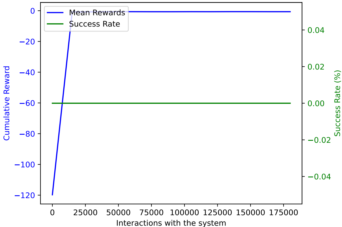
TRPO on AWAKE with DoF: 5 and trained on 180000 samples averaged over 10 validation episodes
