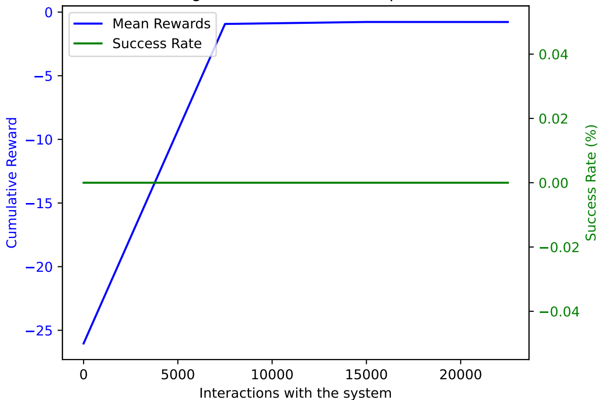
TRPO on AWAKE with DoF: 5 and trained on 22500 samples averaged over 10 validation episodes
