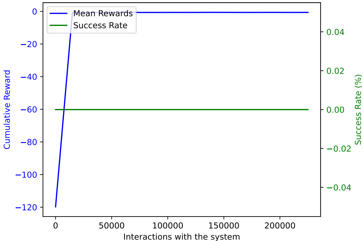
TRPO on AWAKE with DoF: 5 and trained on 225000 samples averaged over 10 validation episodes
