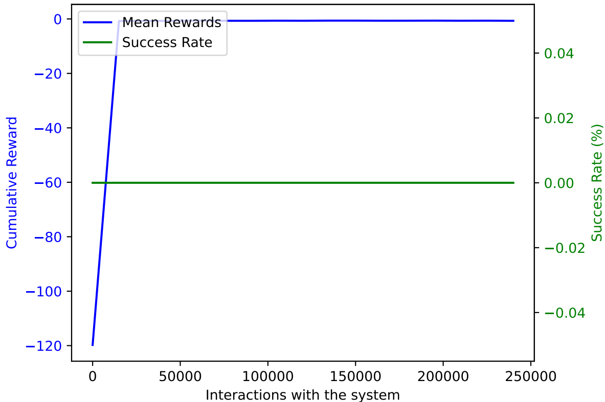
TRPO on AWAKE with DoF: 5 and trained on 240000 samples averaged over 10 validation episodes
