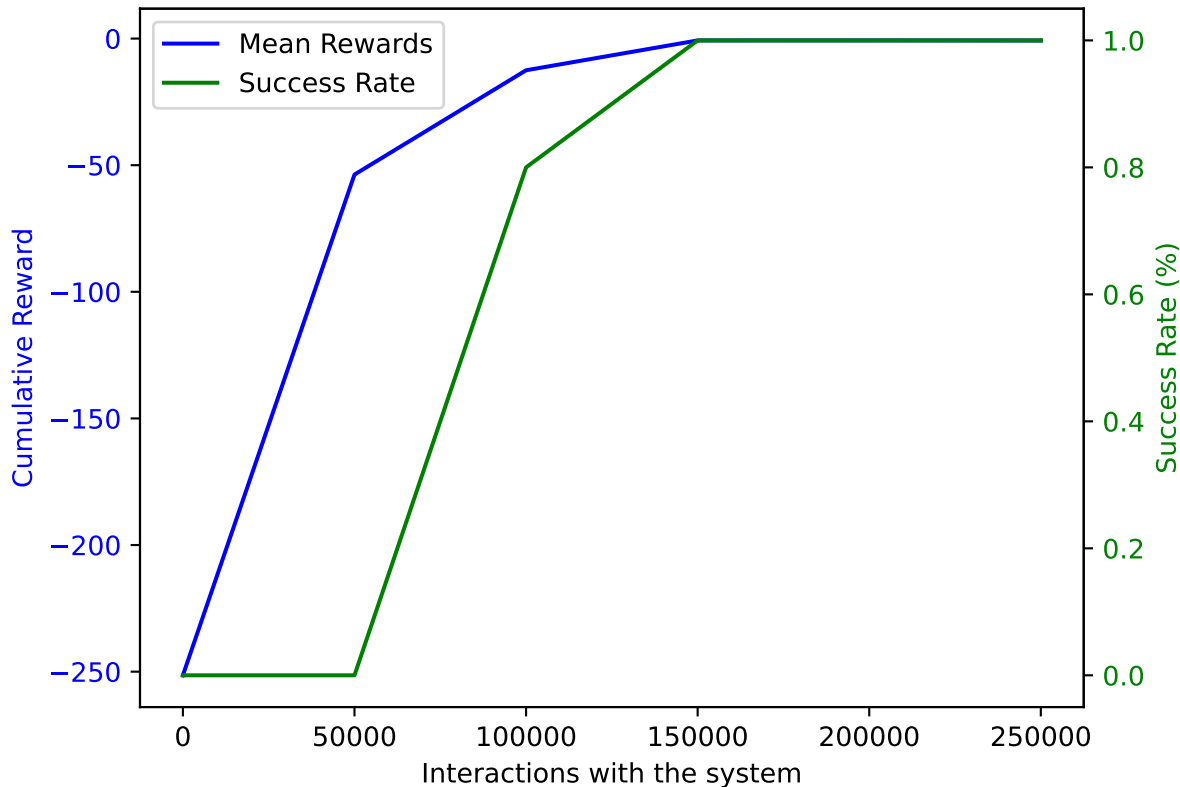
TRPO on AWAKE with DoF: 5 and trained on 250000 samples averaged over 10 validation episodes
