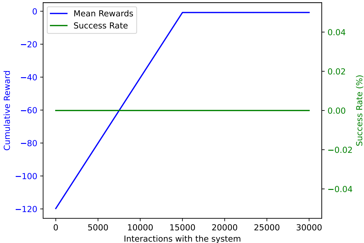
TRPO on AWAKE with DoF: 5 and trained on 30000 samples averaged over 10 validation episodes
