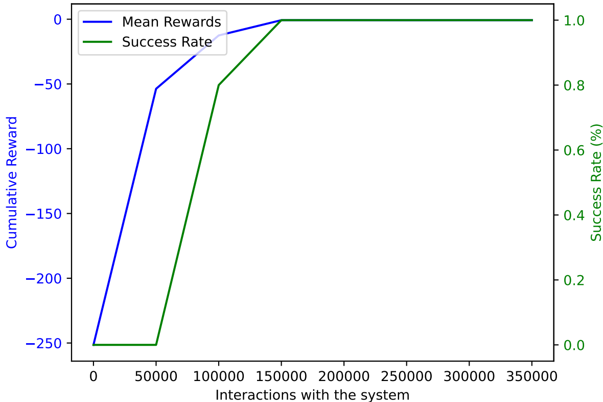
TRPO on AWAKE with DoF: 5 and trained on 350000 samples averaged over 10 validation episodes
