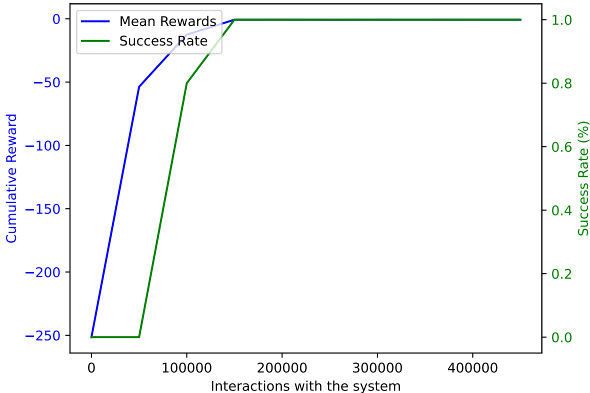
TRPO on AWAKE with DoF: 5 and trained on 450000 samples averaged over 10 validation episodes
