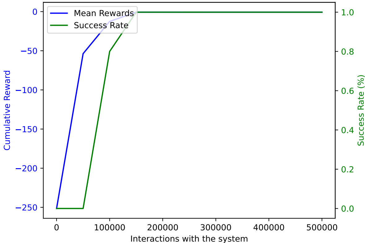
TRPO on AWAKE with DoF: 5 and trained on 500000 samples averaged over 10 validation episodes
