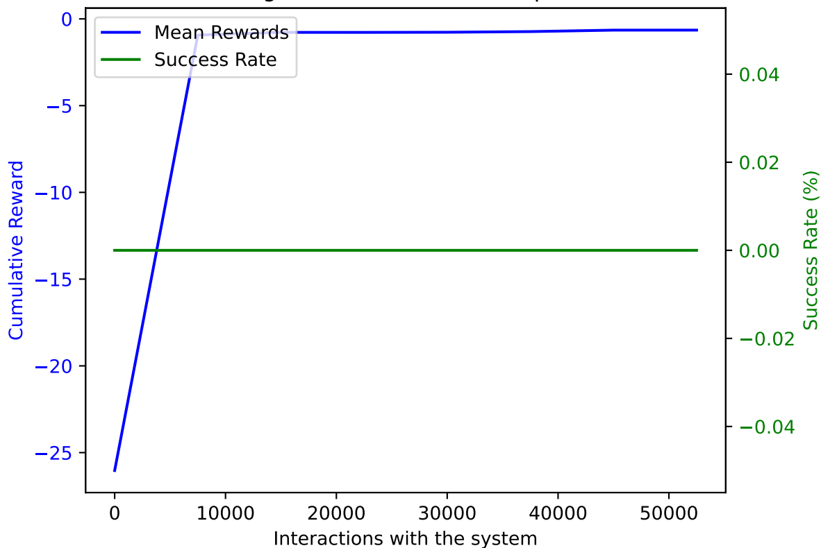
TRPO on AWAKE with DoF: 5 and trained on 52500 samples averaged over 10 validation episodes
