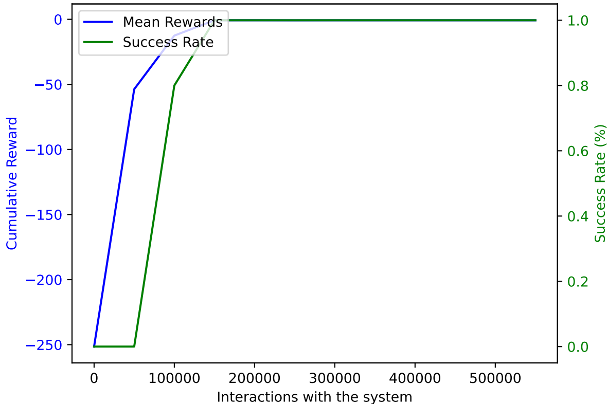
TRPO on AWAKE with DoF: 5 and trained on 550000 samples averaged over 10 validation episodes
