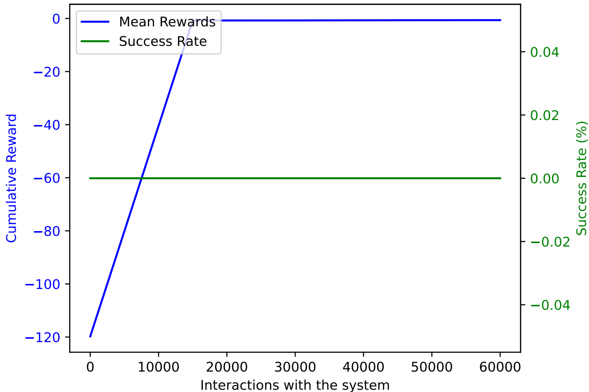
TRPO on AWAKE with DoF: 5 and trained on 60000 samples averaged over 10 validation episodes
