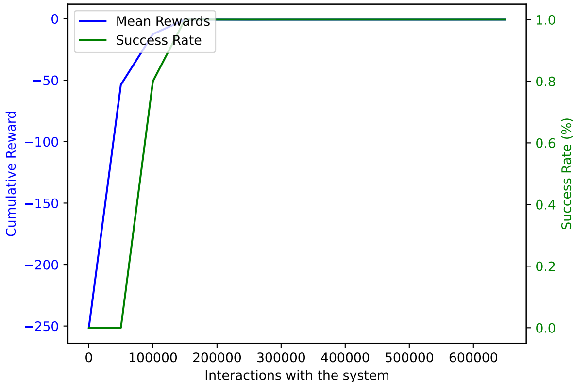
TRPO on AWAKE with DoF: 5 and trained on 650000 samples averaged over 10 validation episodes
