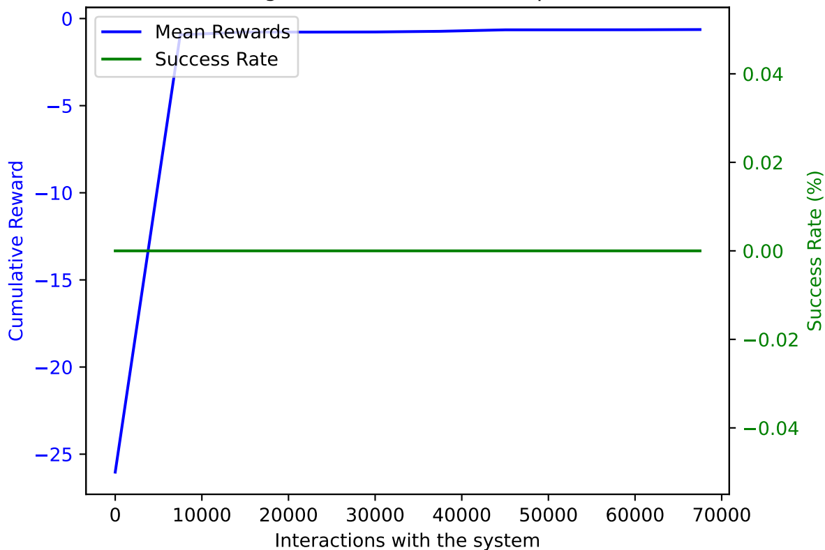
TRPO on AWAKE with DoF: 5 and trained on 67500 samples averaged over 10 validation episodes
