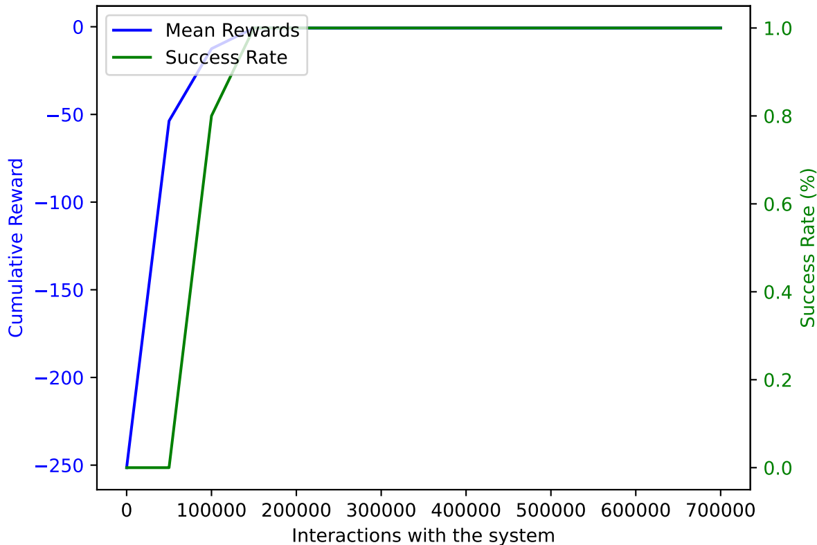
TRPO on AWAKE with DoF: 5 and trained on 700000 samples averaged over 10 validation episodes
