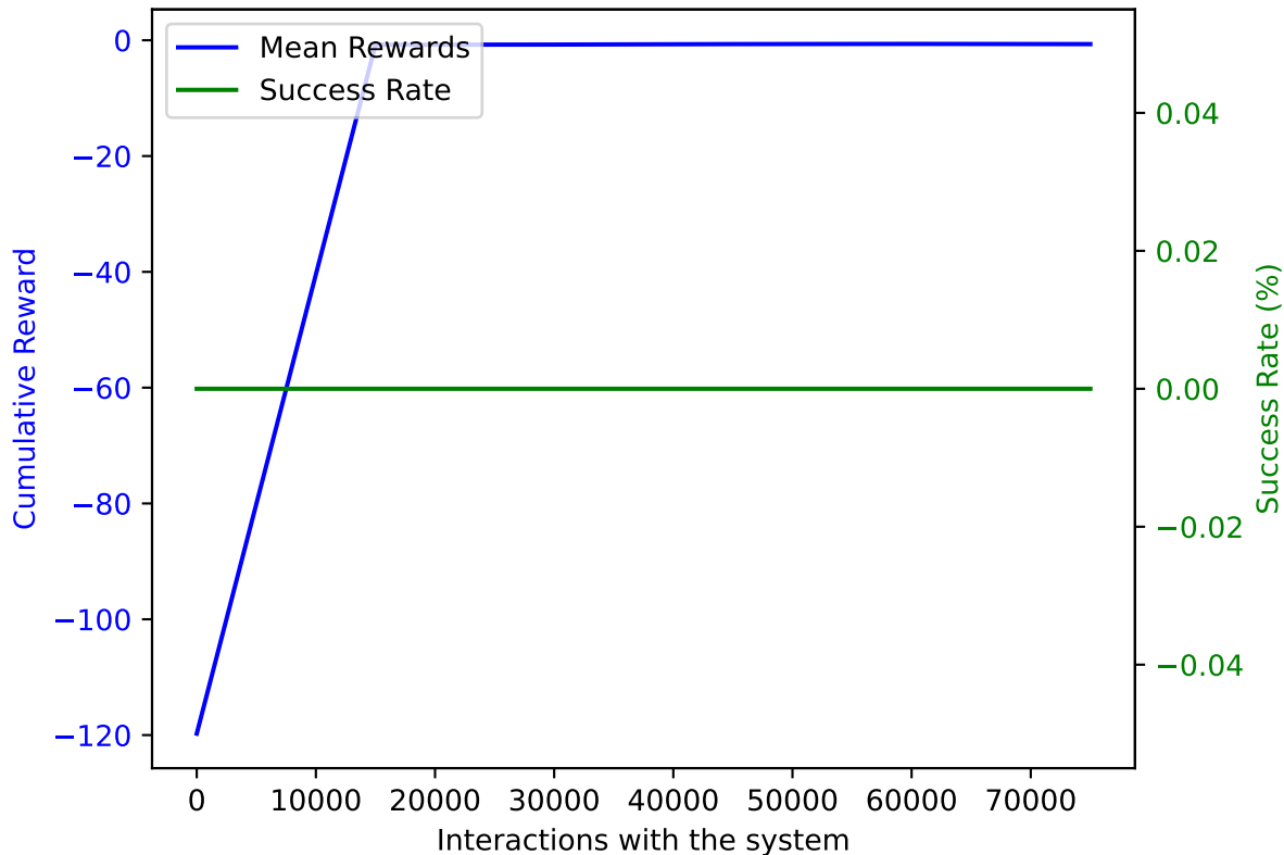
TRPO on AWAKE with DoF: 5 and trained on 75000 samples averaged over 10 validation episodes
