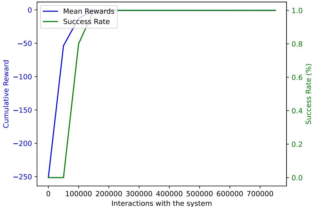
TRPO on AWAKE with DoF: 5 and trained on 750000 samples averaged over 10 validation episodes
