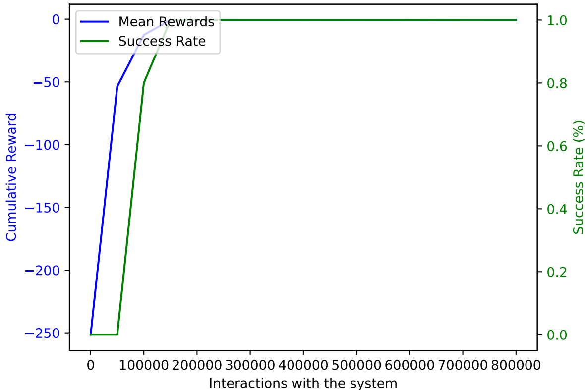
TRPO on AWAKE with DoF: 5 and trained on 800000 samples averaged over 10 validation episodes
