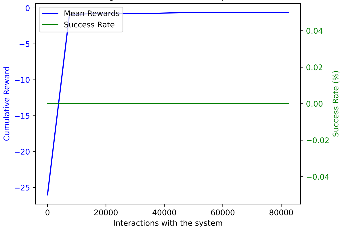
TRPO on AWAKE with DoF: 5 and trained on 82500 samples averaged over 10 validation episodes
